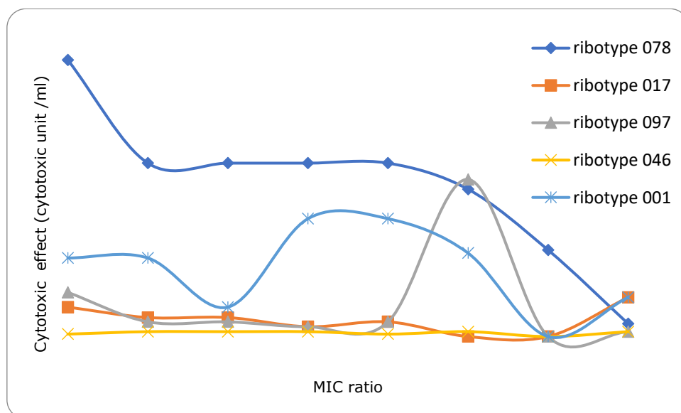
Fig 4: Mean cytotoxic activity (CU/ml) of cell-bound cytotoxin of C. difficile post exposure to vancomycin by all test strains
