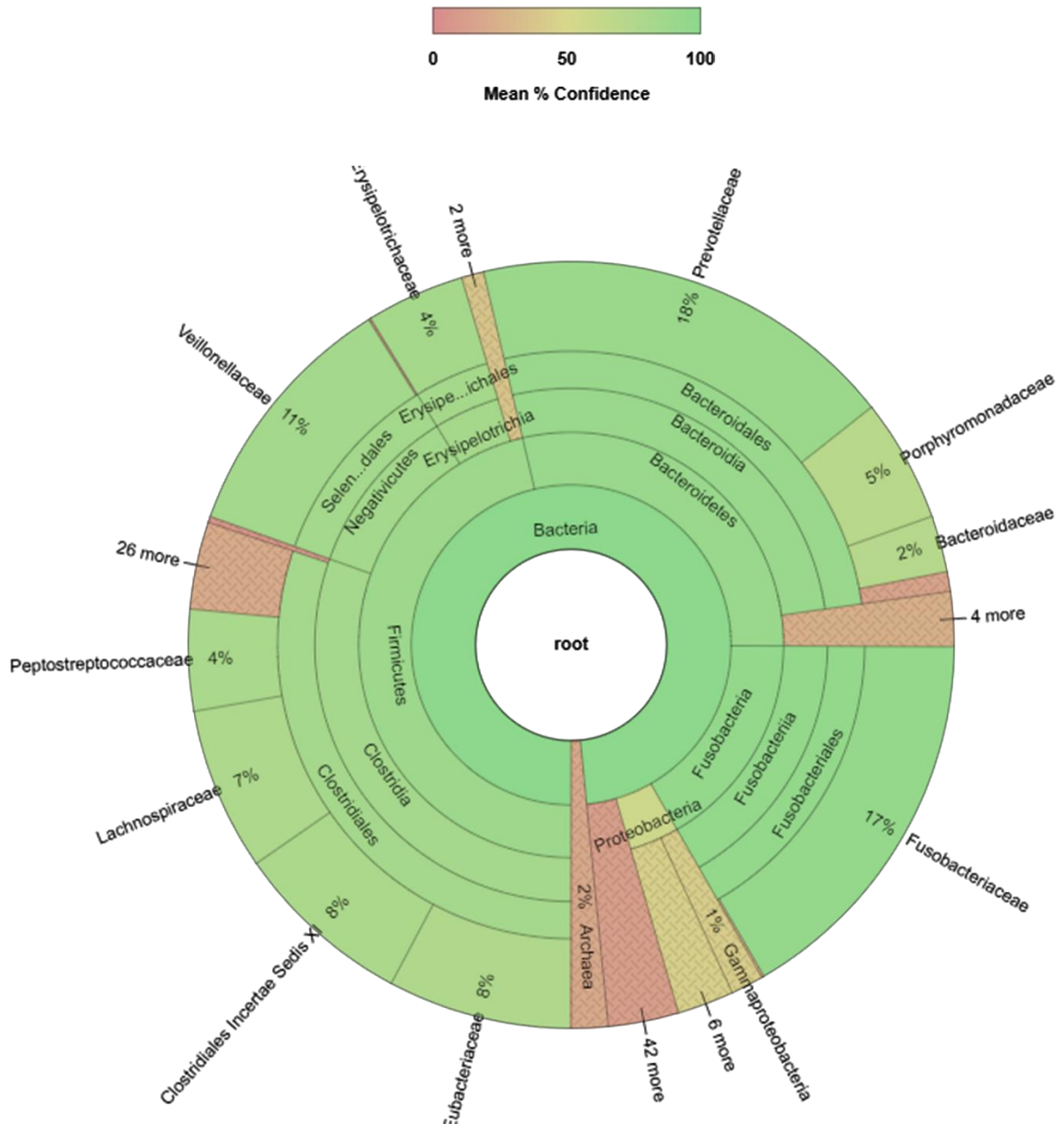
Supplementary Fig 5: Krona chart of sample OIF6 Full names of truncated legends/labels: Eubacteriaceae, Erysipelotrichaceae
