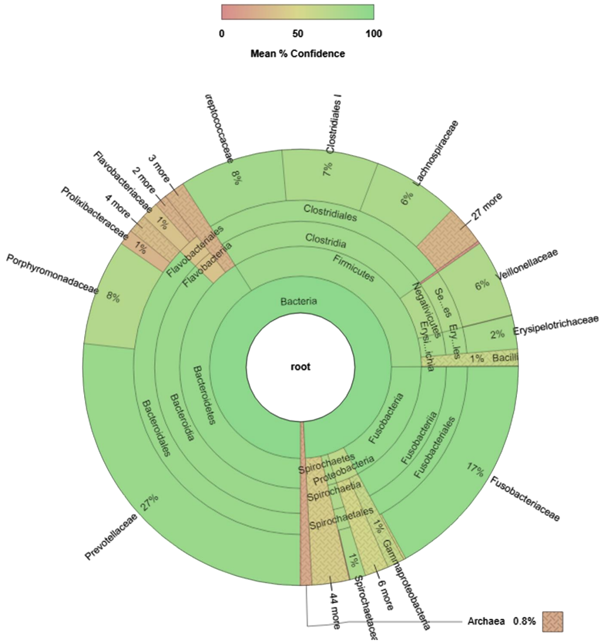
Supplementary Fig 4: Krona chart of sample OIF5 Full names of truncated legends/labels: Peptostreptococcaceae, Clostridiales Incertae Sedis XI
